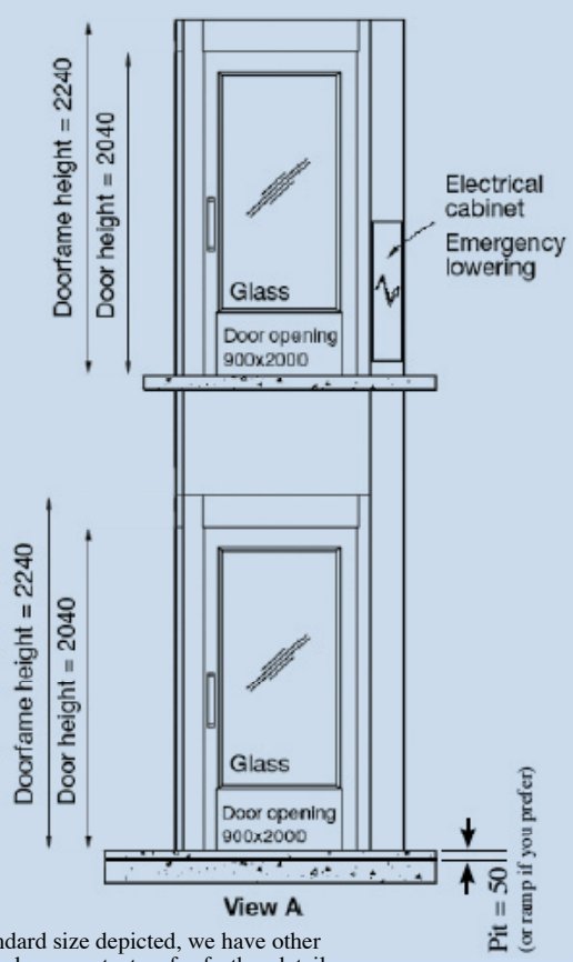
standard layout (section view)*
