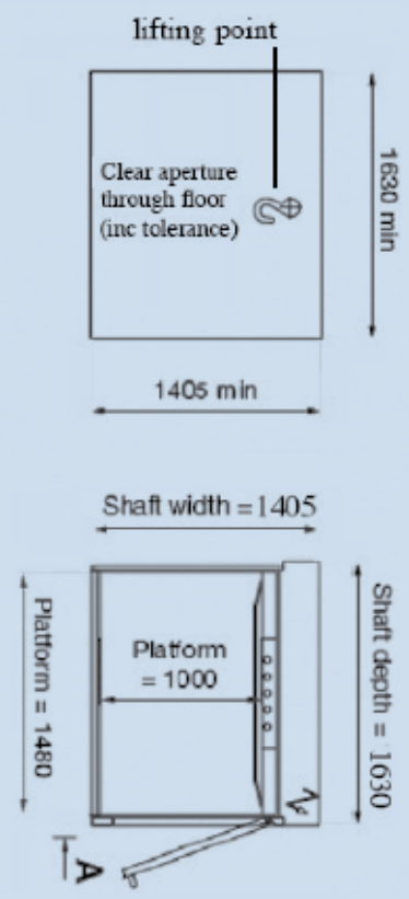
standard layout (plan view)*
