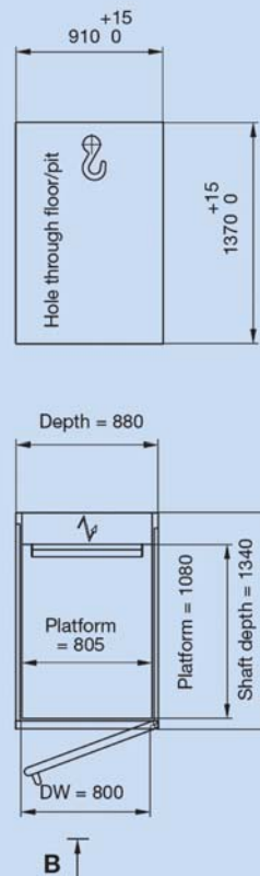
standard layout (plan view)*
