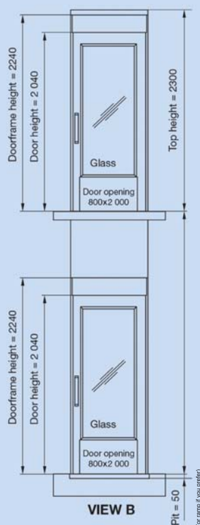
standard layout (section view)*
