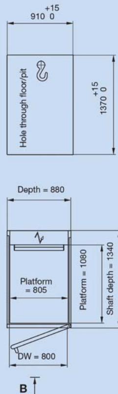
standard layout (plan view)*
